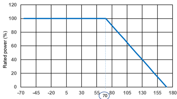
Figure 1. : Power derating curve at ambient temperature
